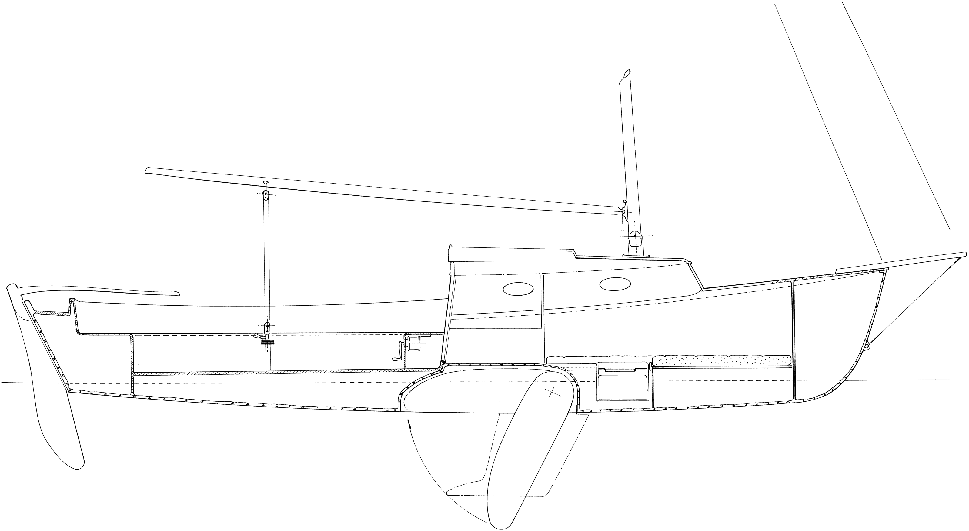
NORSEBOAT 21.5 INBOARD PROFILE
